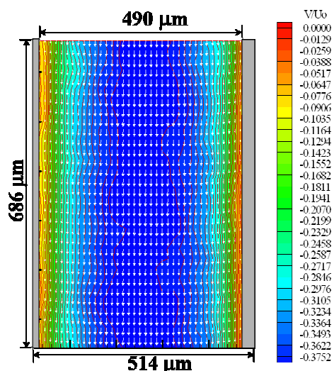
Fig. 5. Streamwise mean velocity field of blood flow.
