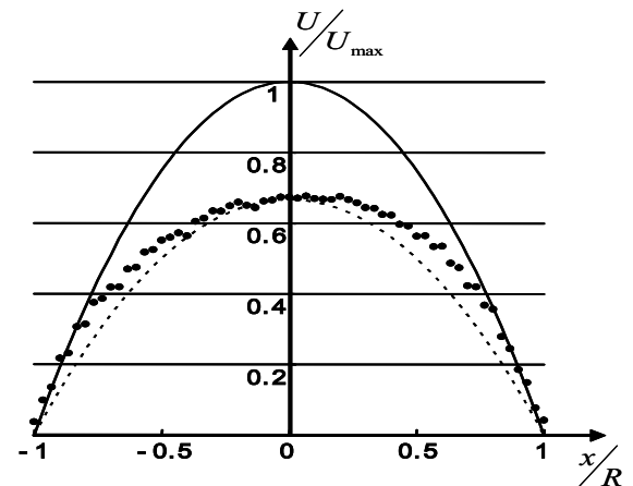
Fig. 2. Streamwise mean velocity profile.
