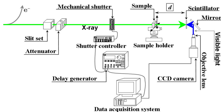
Fig. 1. Schematics of synchrotron X-ray PIV.
